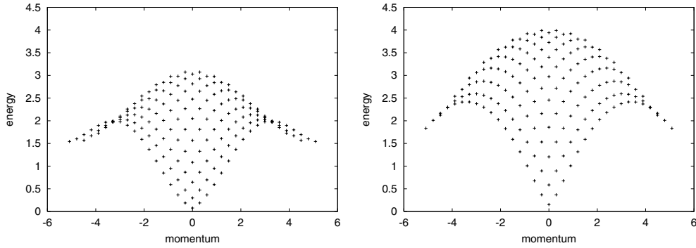
Figure 8. The coloron( \sigma type)–coloron( \sigma type) excitation spectrum calculated for N = L = 21 , and c = 10 (left) and c = 1 (right).
