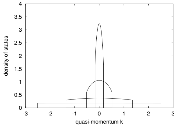
Figure 1. The density of state in k -space for the ground state. The distribution changes gradually from a histogram to a narrow peak for the coupling from strong to weak. The figure is plotted for N = L = 41 and c = 10, 1, 0.1, 0.01 .
