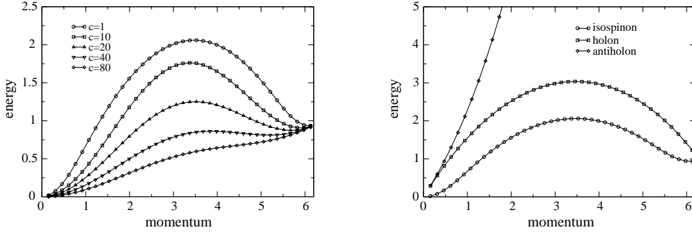
Fig. 3 – Dispersion relations of the isospin for different coupling constants (left); the curves from top to bottom correspond to c = 1, 10, 20, 40 , and 80 , respectively. Right: dispersion of antiholon, holon, and isospin, for c = 1 ( L = 20, N = 40 ).
